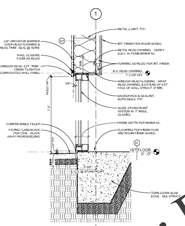
B1 STOREFRONT HEAD & SILL 1 1/2" = 1'-0"
