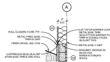
E6 METAL PANEL TERM AT CMU WALL 3/4" = 1'-0"
