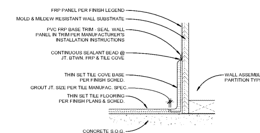
D3 SECTION DETAIL @ RR TILE BASE 3" = 1'-0"
