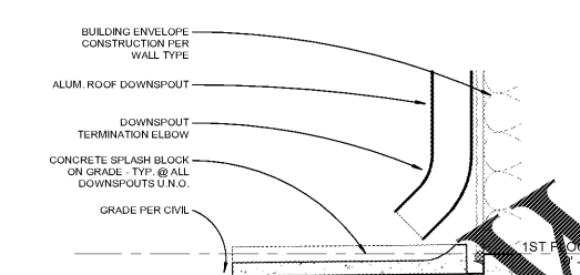
C3 DETAIL @ DOWNSPOUT TERMINATION 1 1/2" = 1'-0"
