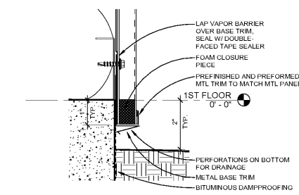
B4 TYP WALL TERM DETAIL 0" = 1'-0"
