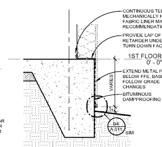
A5 PHASE 4 - WALL TERM. @ GRADE DROP 3/4" = 1'-0"
