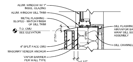
C6 WINDOW SILL FLASHING @ CMU 1 1/2" = 1'-0"
