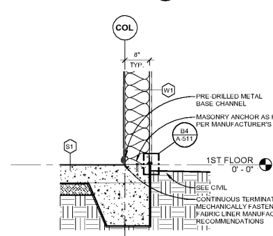
A4 TYP WALL TERMINATION @ SOG 3/4" = 1'-0"
