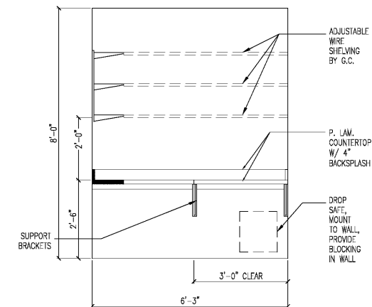
6 OFFICE ELEVATION A-100.1 1/2"=1'-0"
