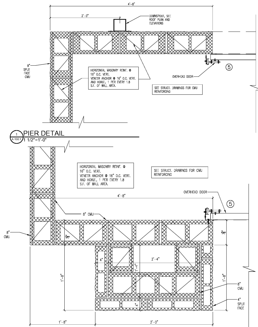
2 PIER DETAIL A-100.1 1/2"=1'-0"
