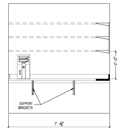
5 OFFICE ELEVATION A-100.1 1/2"=1'-0"
